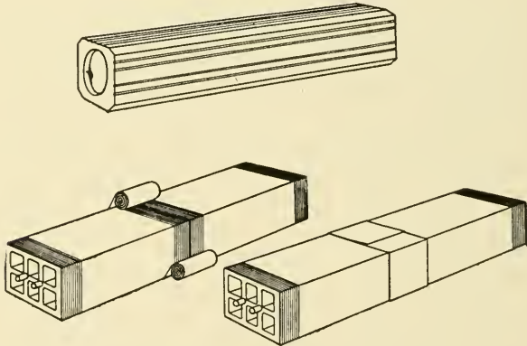
Fig. 47. Single- and Multiple-Duct Tile Conduits
